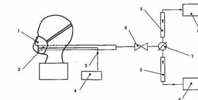
Figure 3 Schematic diagram of the inspiratory and expiratory resistance detection devices
