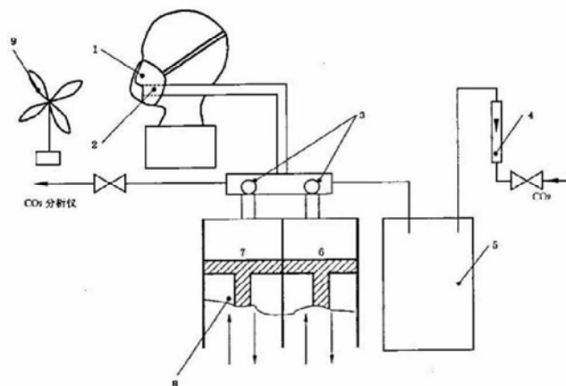
Figure 5: Schematic of a dead space detection device
