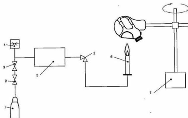
Figure 6: Diagram of a flammability detection device
