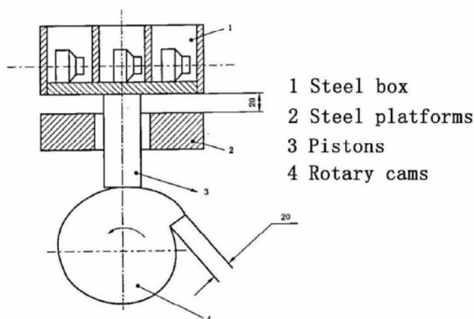
Figure 1: Schematic of the vibration test device
